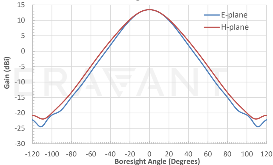
Simulated Antenna Patterns @ 60 GHz
