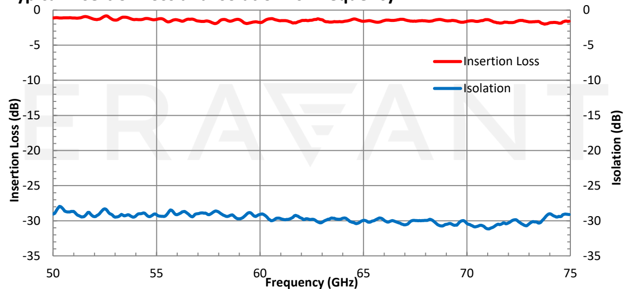
Typical Insertion Loss and Isolation vs. Frequency
