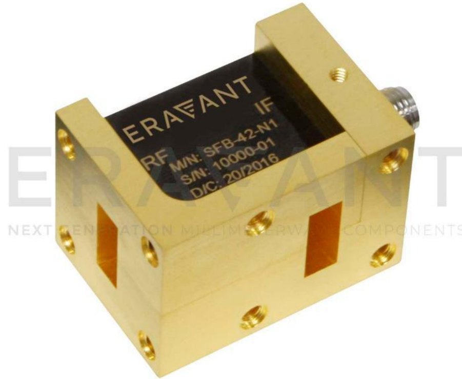
Balanced Mixers SFB-42-N1
