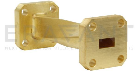
Waveguide Twist SWB-42090-TB
