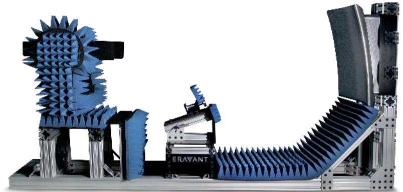
Open Bed Compact Antenna Test Range System
