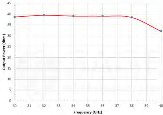
Typical Output Power Psat Vs. Frequency Bias = +48 V DC / 2 A
