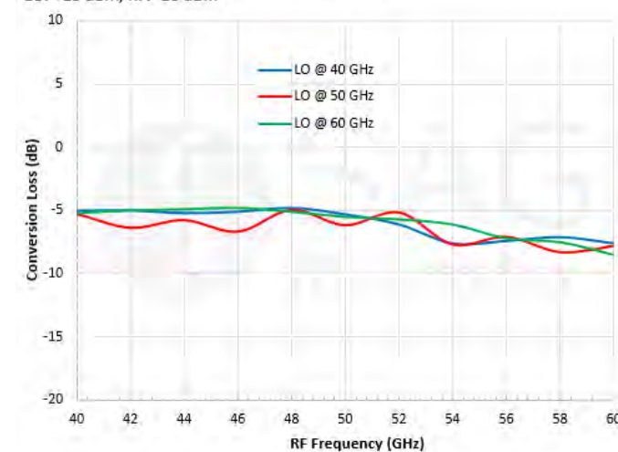
Typical Conversion Loss vs. Frequency
