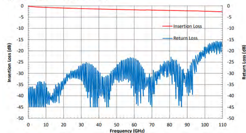
Typical Insertion Loss & Return Loss vs. Frequency
