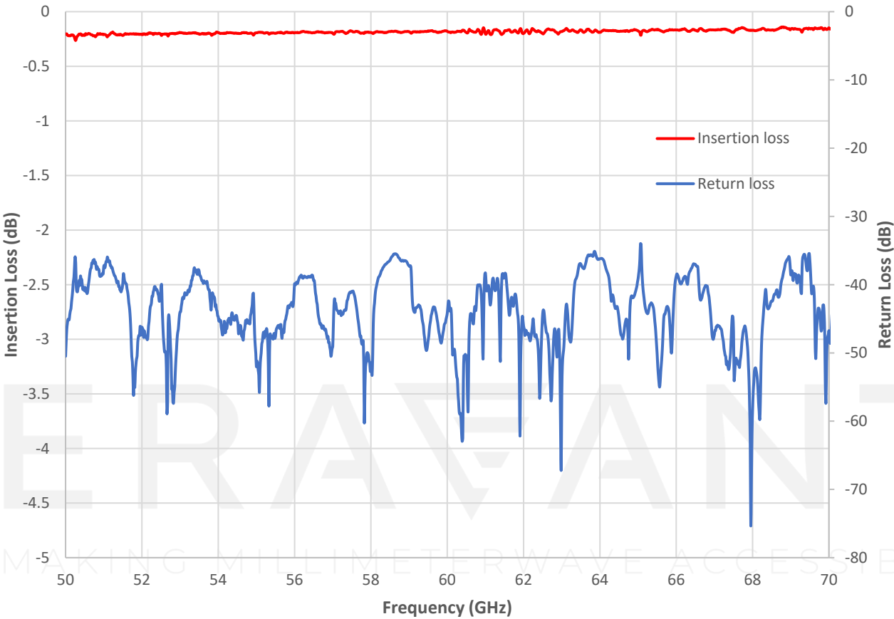
Measured Insertion Loss and Return Loss Vs Frequency
