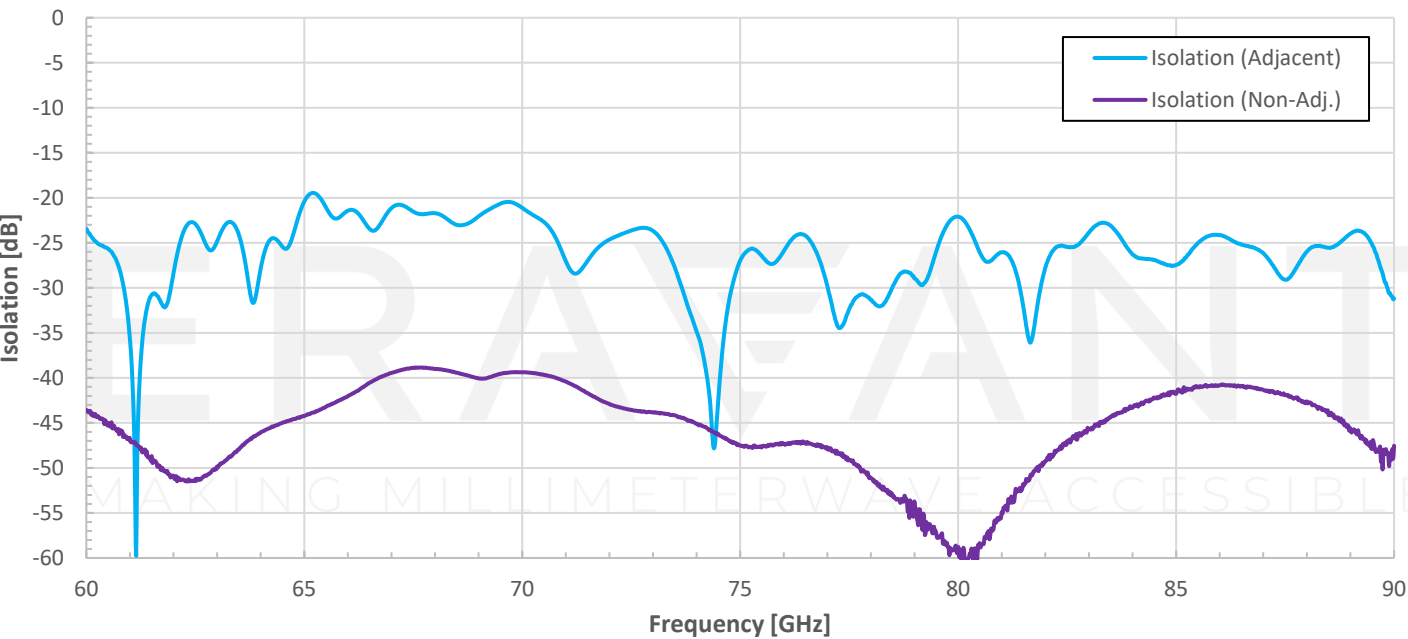
Typical Measured Isolation vs Frequency
