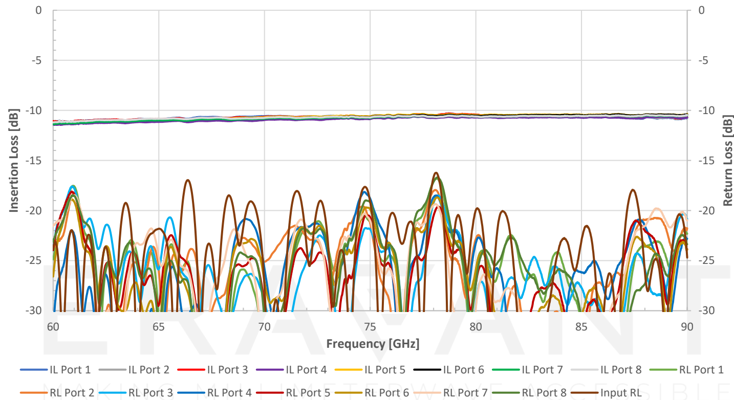
Typical Measured Insertion and Return Loss vs Frequency
