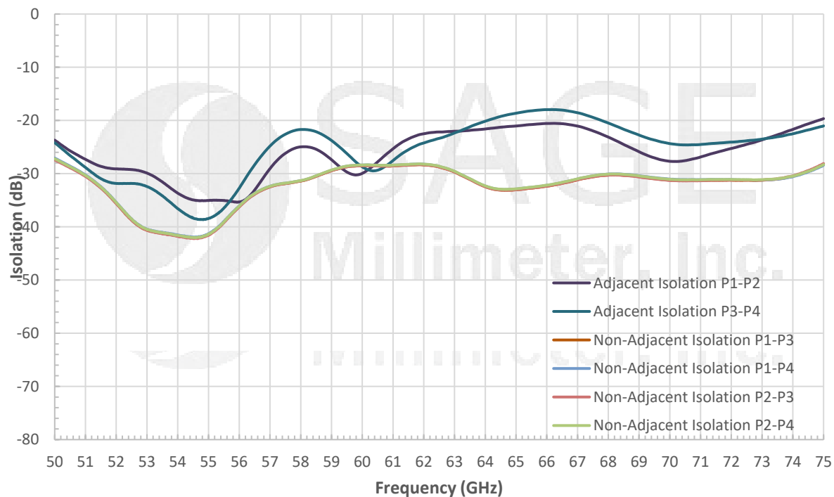
Measured Isolation Vs Frequency
