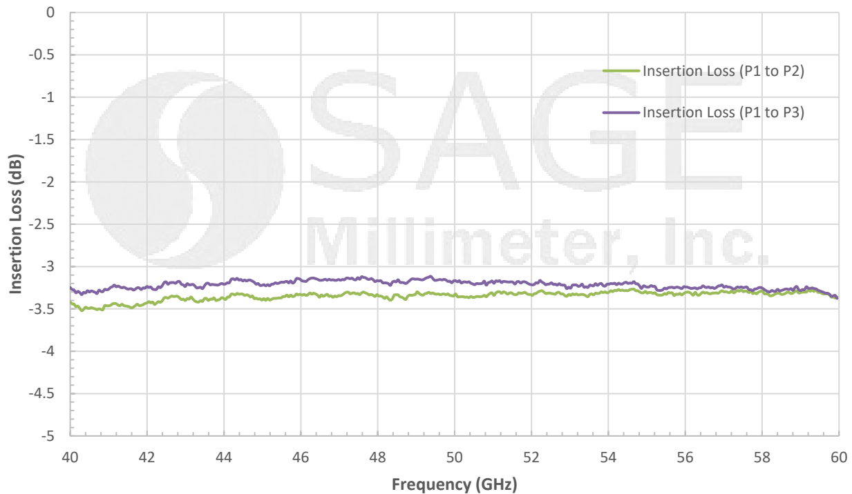
Typical Measured Insertion Loss Vs Frequency
