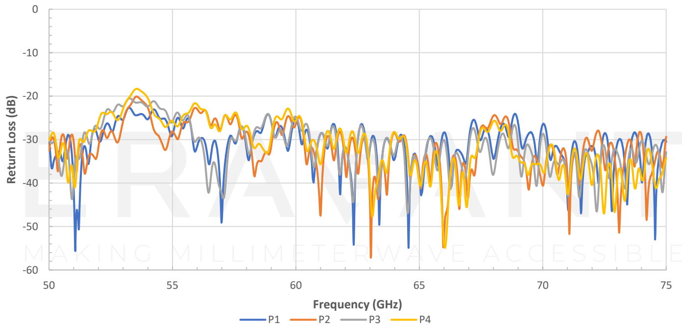
Typical Measured Return Loss vs Frequency
