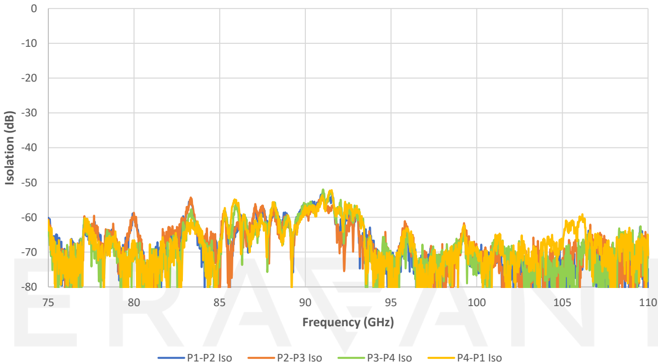
Typical Measured Isolation vs Frequency
