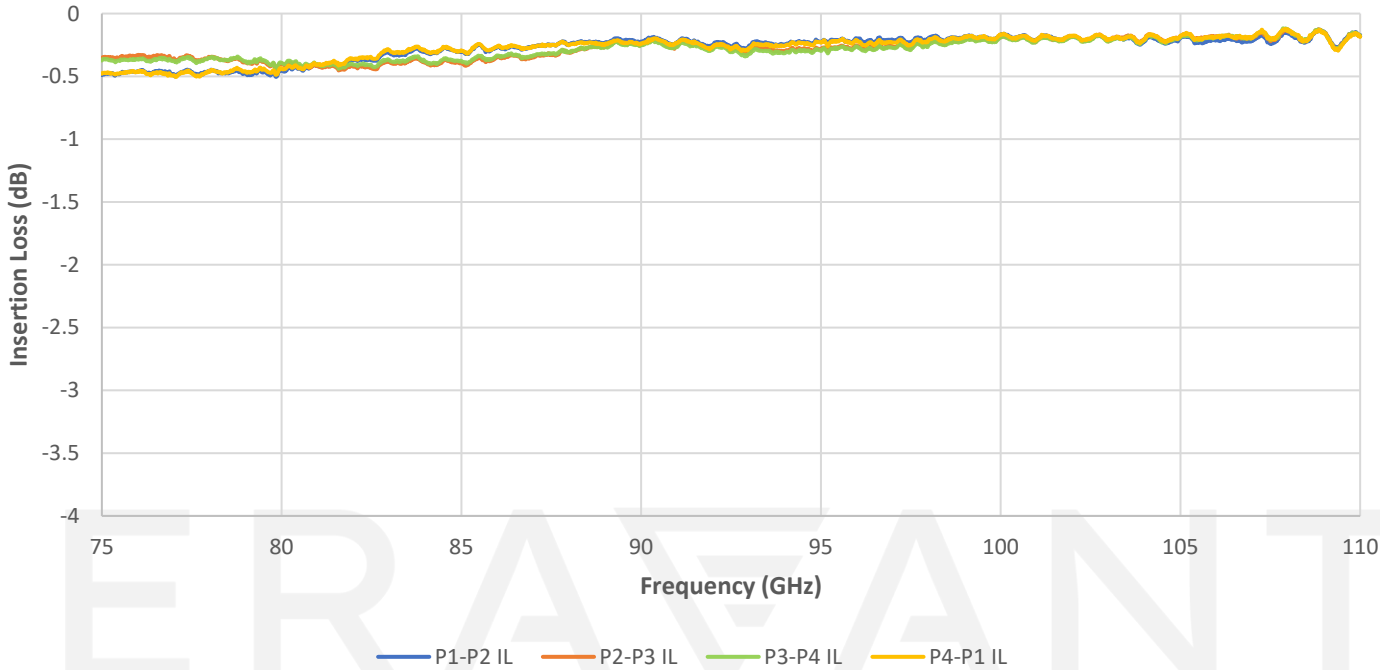
Typical Insertion Loss vs Frequency
