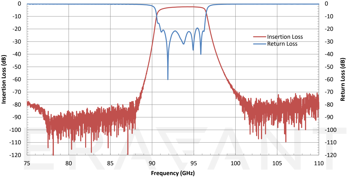
Insertion Loss and Return Loss vs. Frequency
