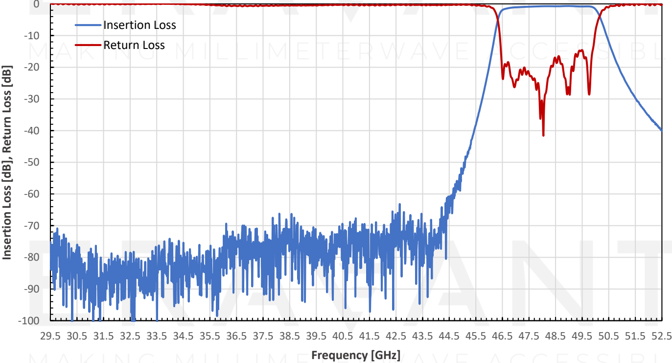
Typical Rejection vs. Frequency
