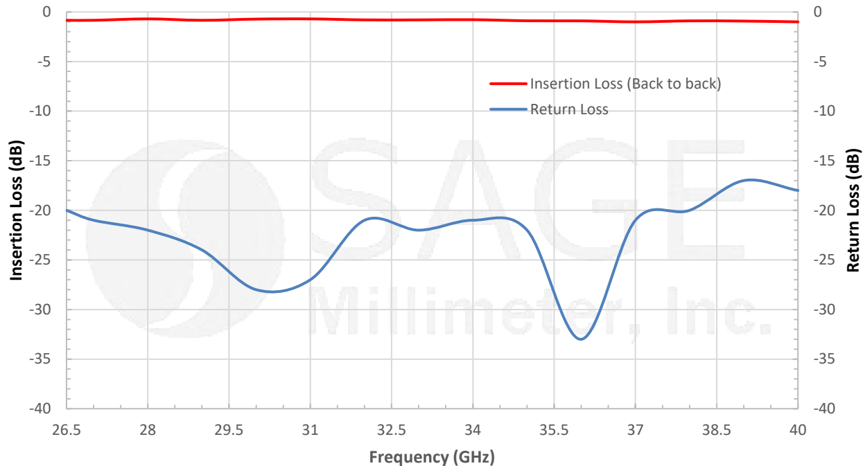
Typical Return Loss & Back to Back Insertion Loss vs. Frequency
