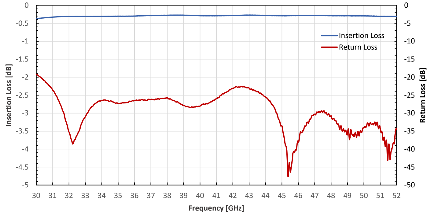
Typical Performance vs. Frequency (Extended Bandwidth, Single Unit)
