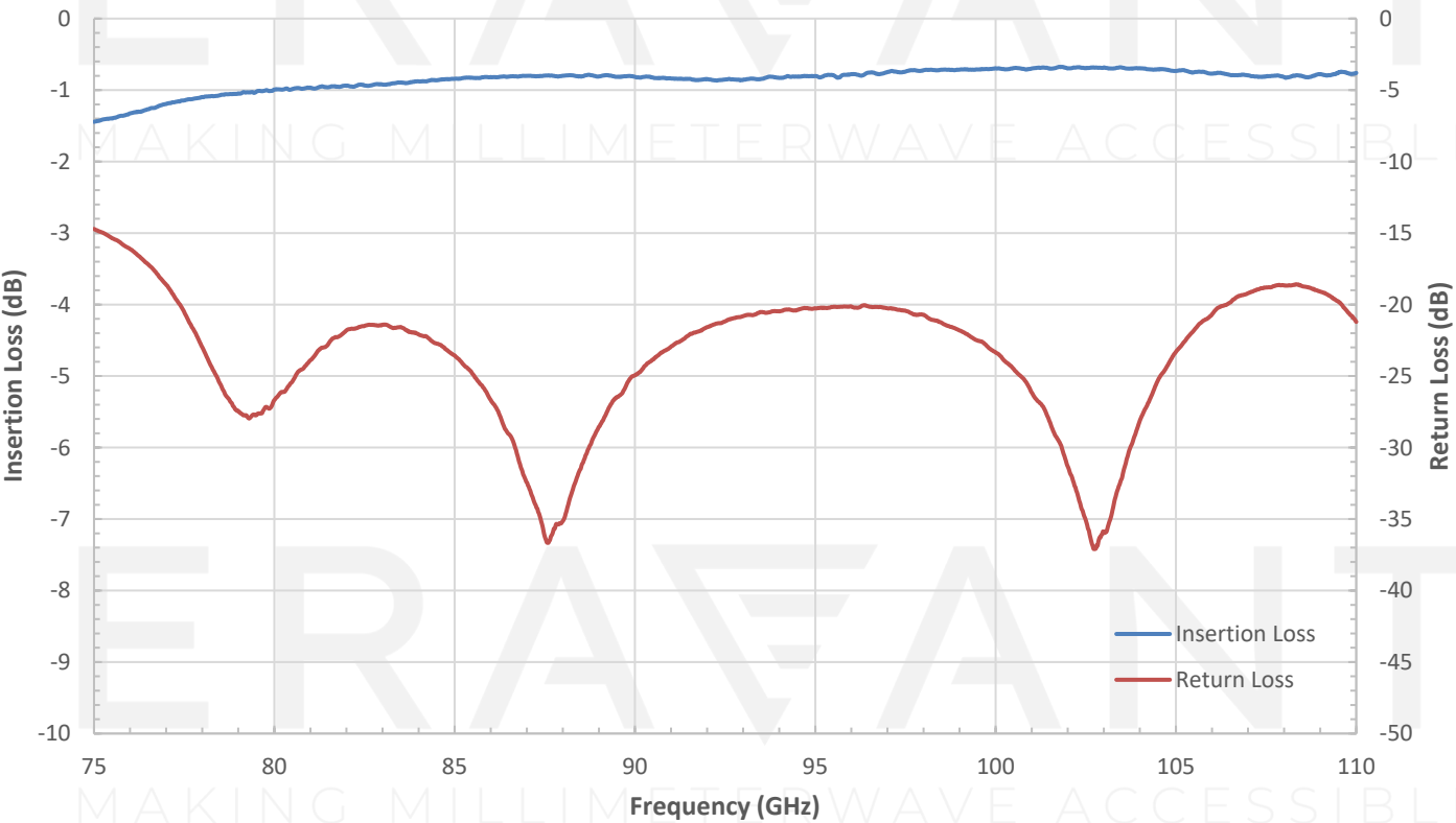
Typical Measured Performance vs Frequency (Single Unit)
