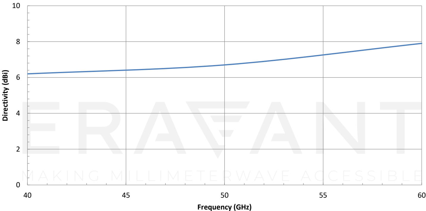
Simulated Directivity vs. Frequency
