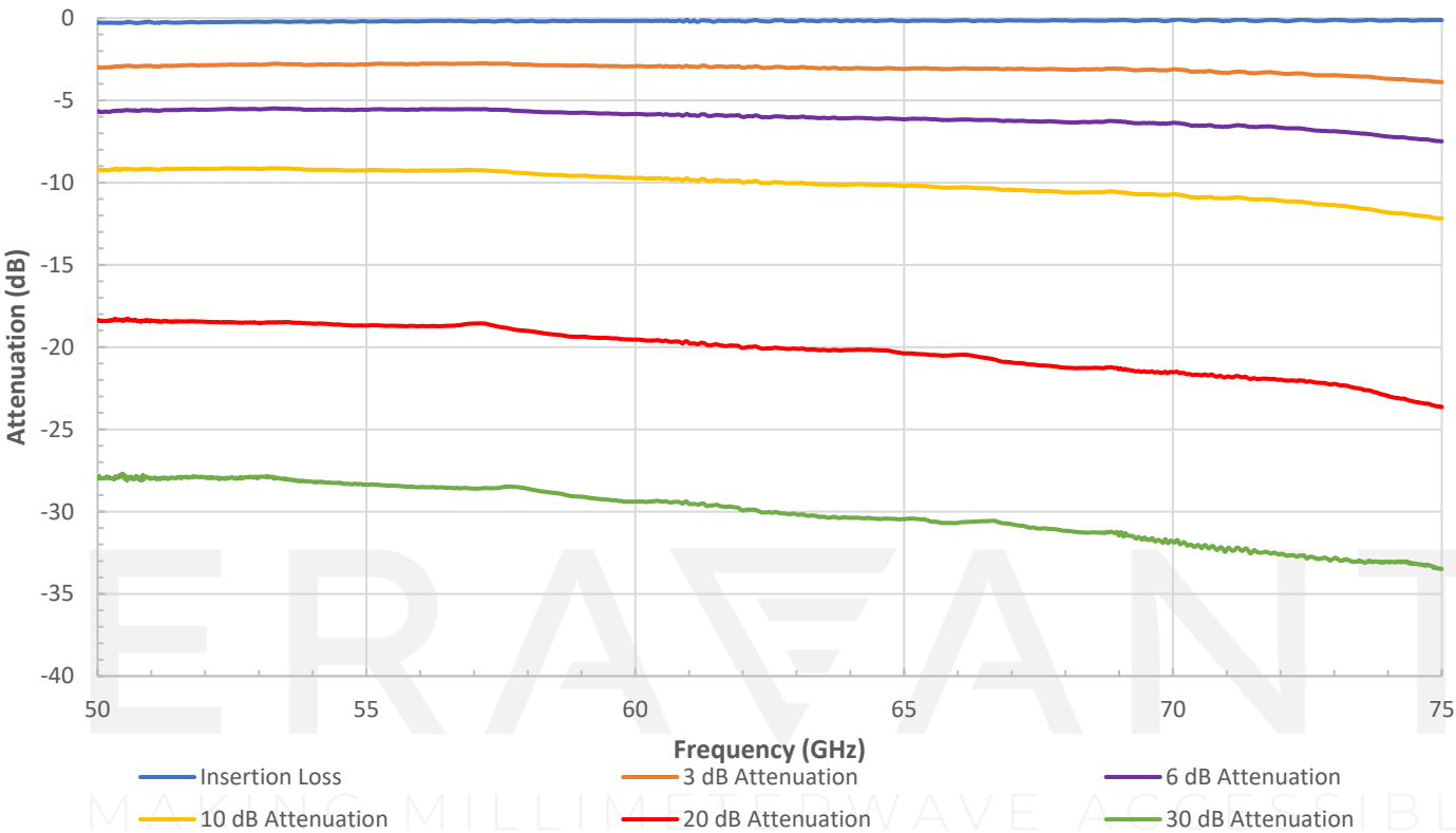
Typical Measured Attenuation vs Frequency
