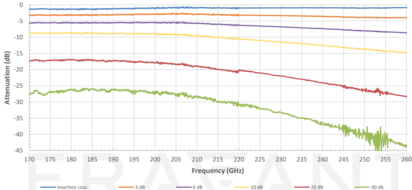
Typical Measured Attenuation vs Frequency
