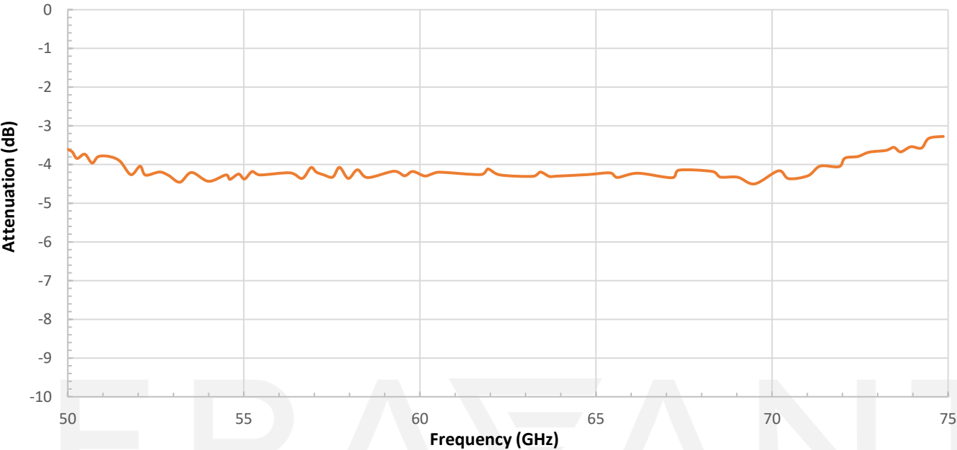
Typical Attenuation vs. Frequency
