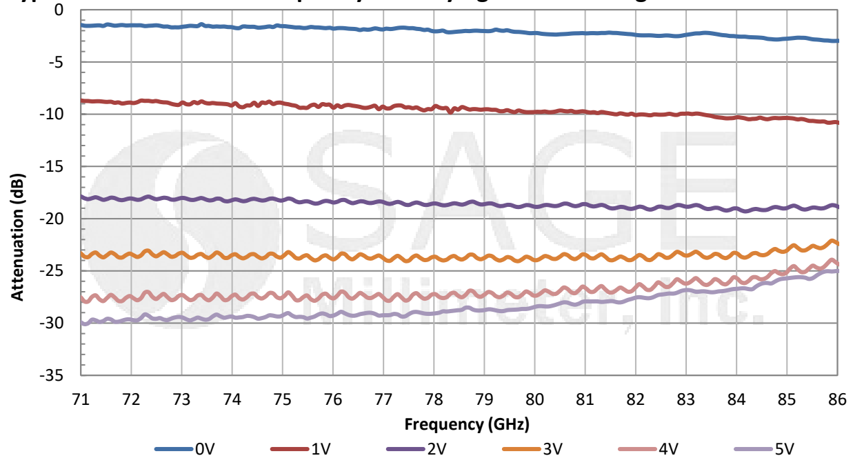
Typical Attenuation vs. Frequency for Varying Control Voltage
