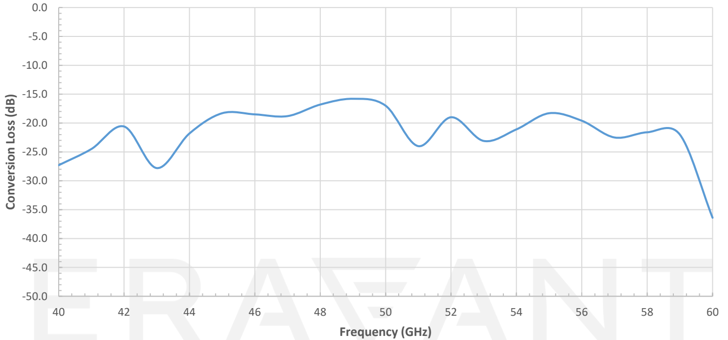
Typical Conversion Loss vs. Frequency
