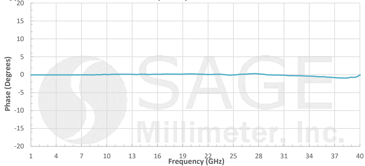
Typical Phase Unbalance vs. Frequency
