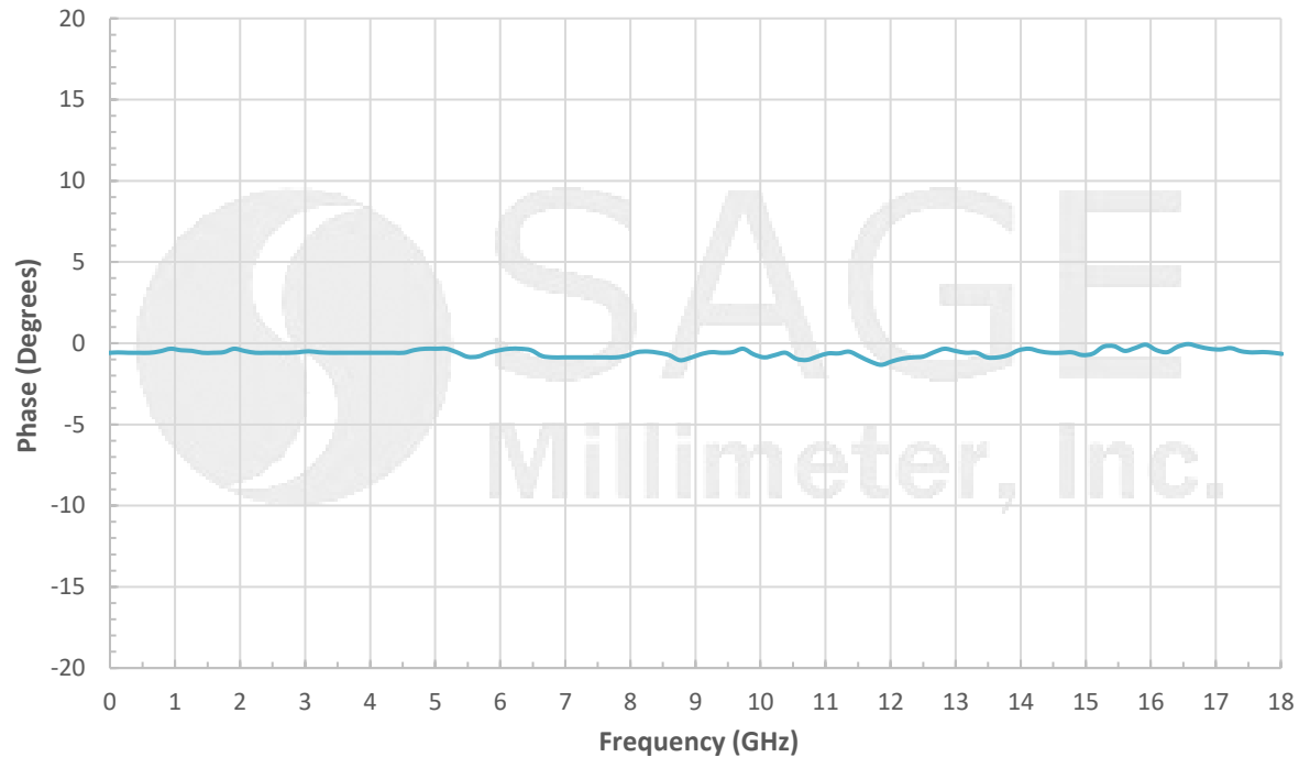
Typical Phase Unbalance vs. Frequency
