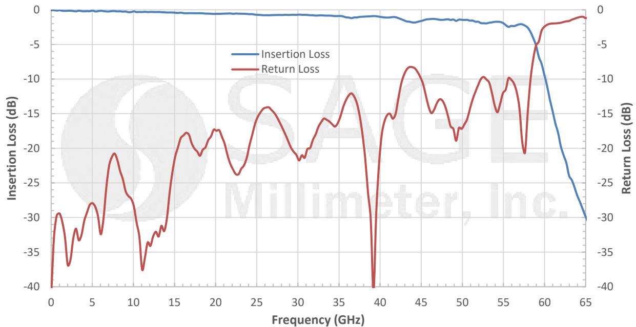
Typical Insertion and Return Loss vs Frequency
