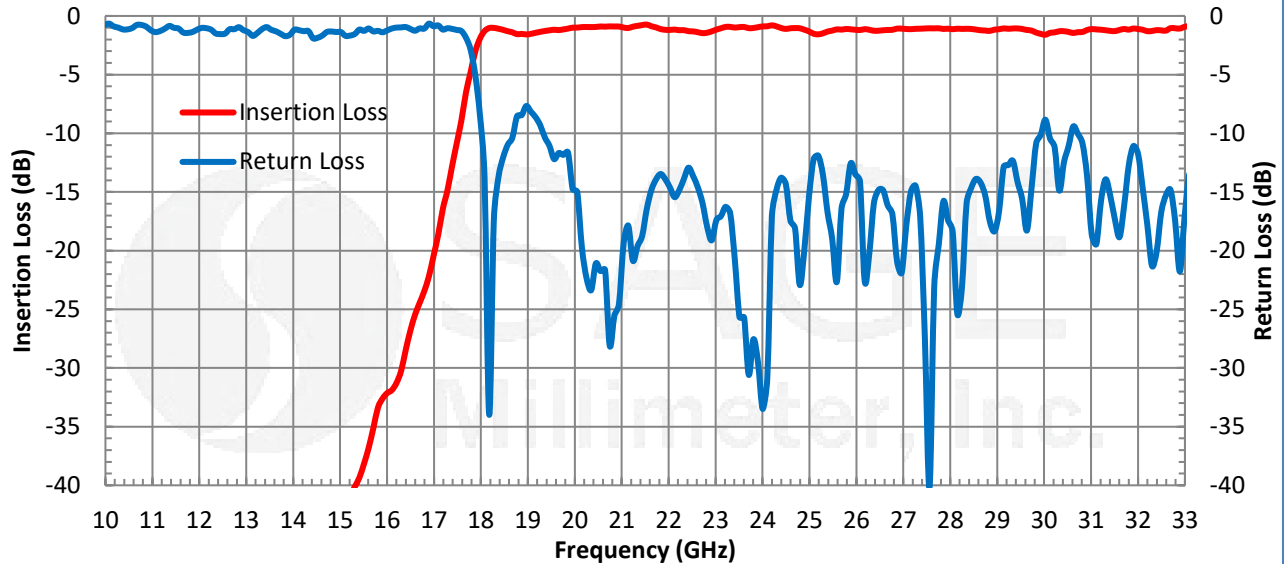
Typical Insertion and Return Loss vs. Frequency
