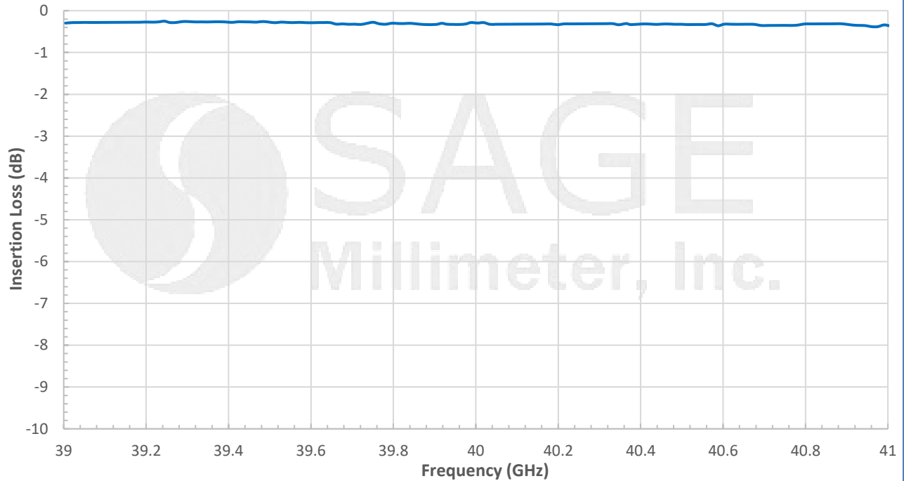
Measured Insertion Loss vs. Frequency
