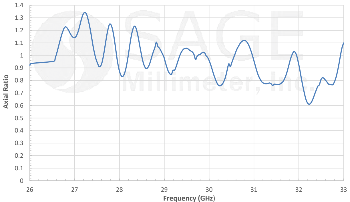
Typical Axial Ratio vs Frequency
