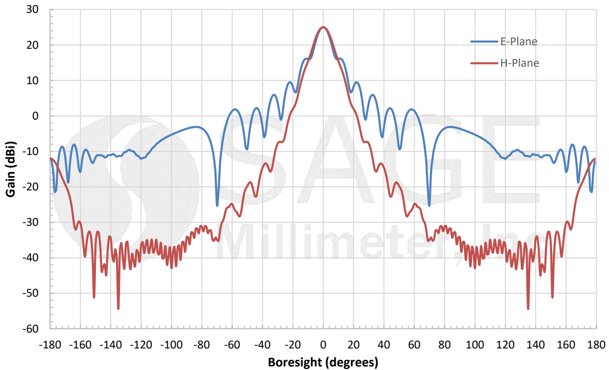
Simulated Antenna Patterns @ 33.5 GHz
