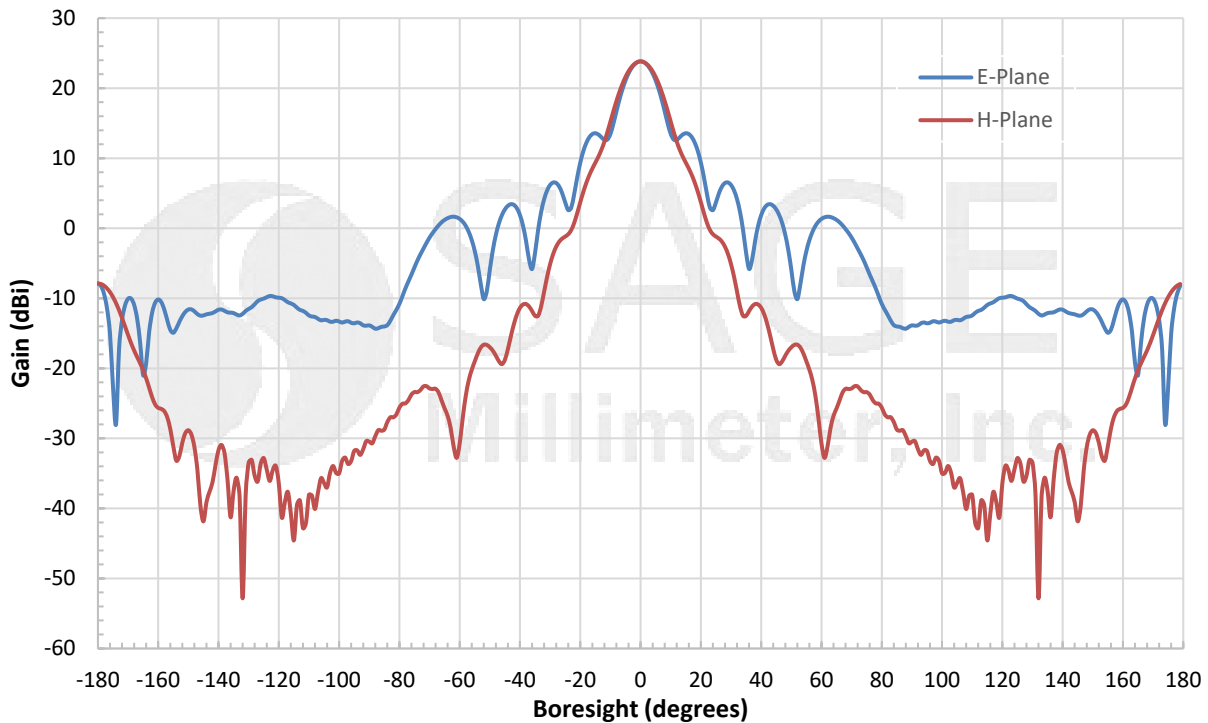
Simulated Antenna Patterns @ 33.5 GHz
