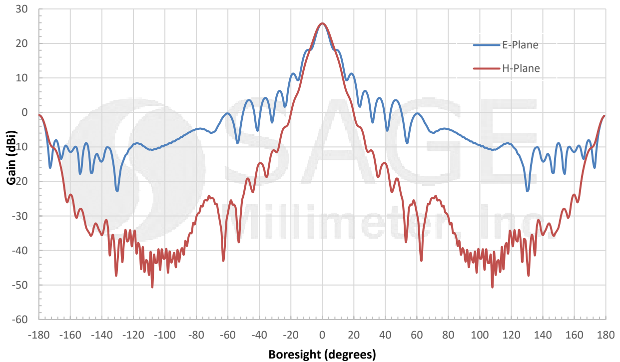
Simulated Antenna Patterns @ 60 GHz
