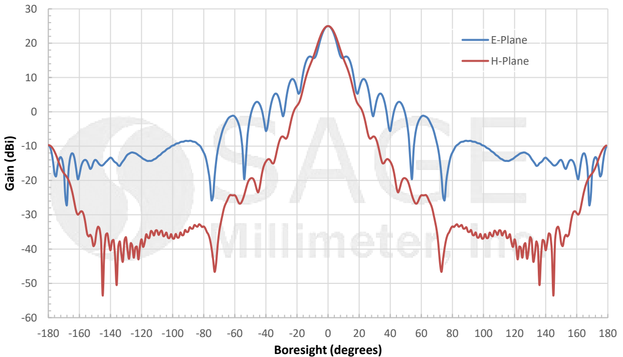
Simulated Antenna Patterns @ 62.5 GHz
