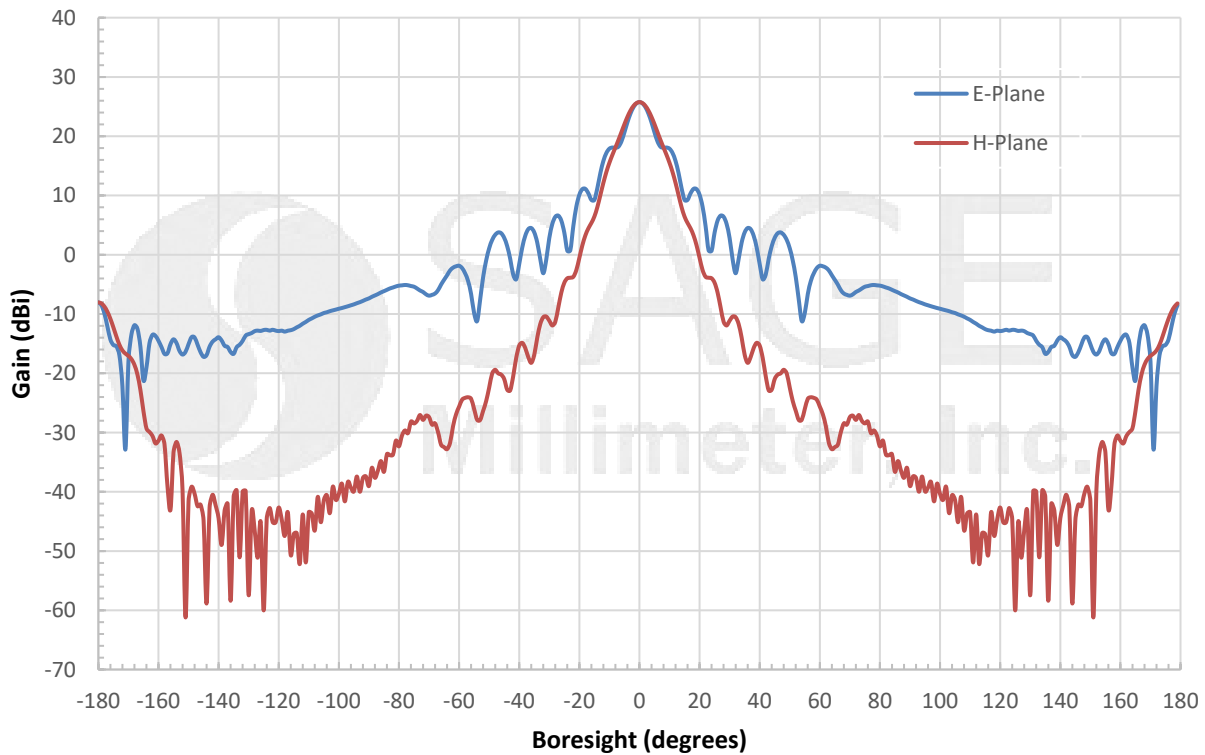
Simulated Antenna Patterns @ 90 GHz
