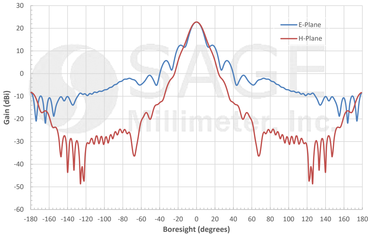
Simulated Antenna Patterns @ 62.5 GHz
