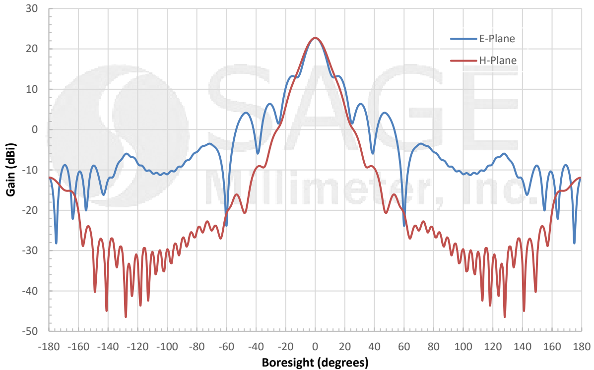
Simulated Antenna Patterns @ 27 GHz
