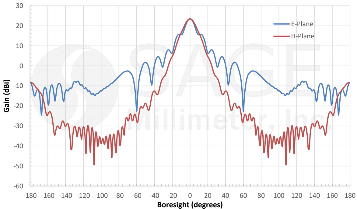
Simulated Antenna Patterns @ 27 GHz
