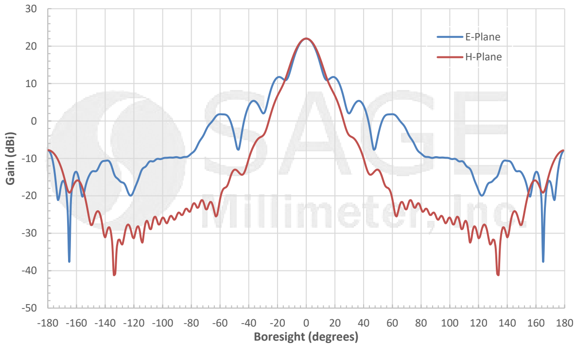
Simulated Antenna Patterns @ 75 GHz
