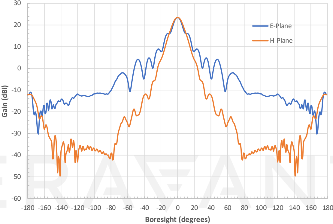
Simulated Antenna Patterns @ 220 GHz
