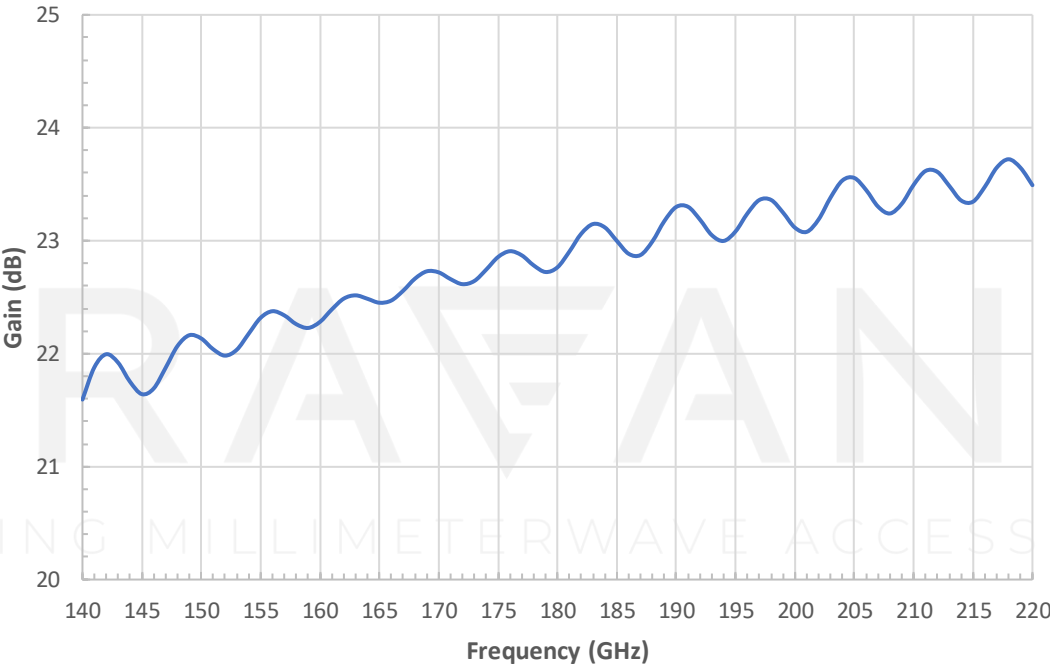
Simulated Gain vs. Frequency
