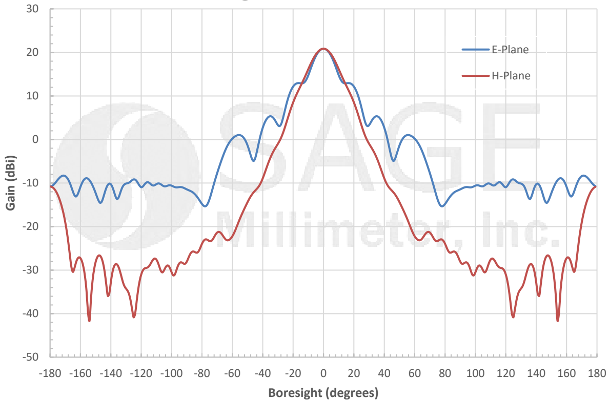
Simulated Antenna Patterns @ 26.5 GHz
