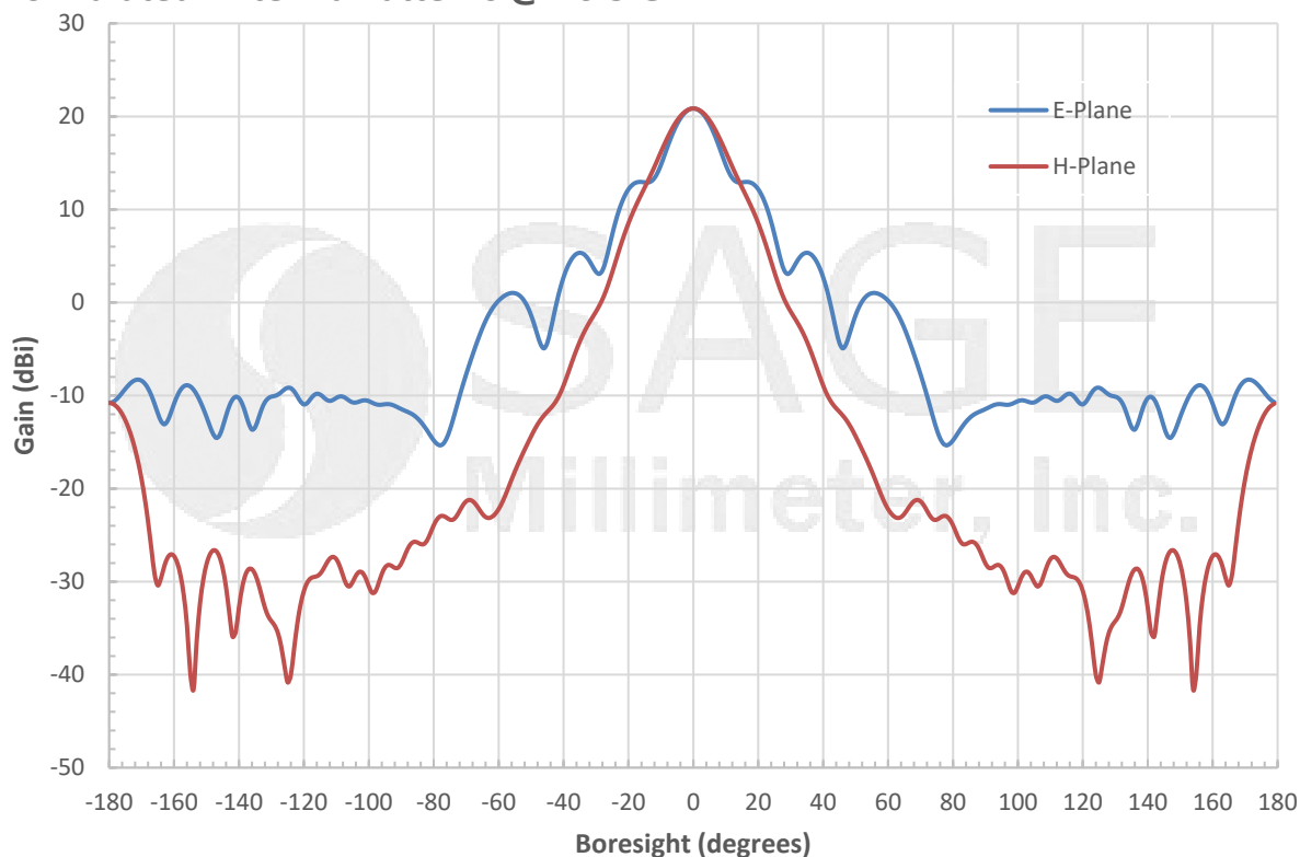
Simulated Antenna Patterns @ 26.5 GHz
