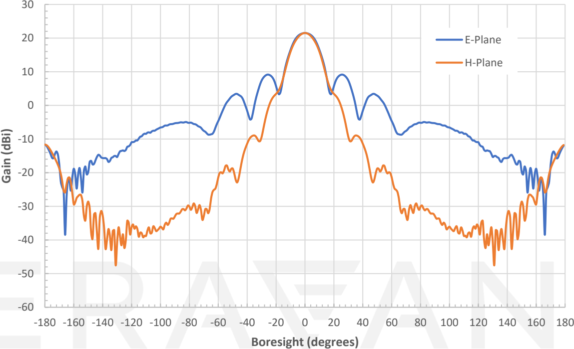
Simulated Antenna Patterns @ 220 GHz
