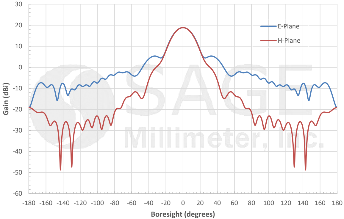
Simulated Antenna Patterns @ 33 GHz
