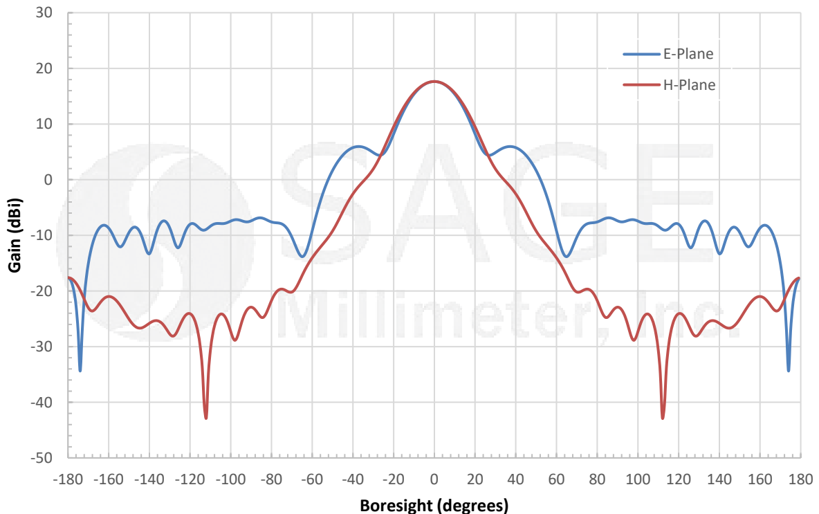
Simulated Antenna Patterns @ 33.25 GHz
