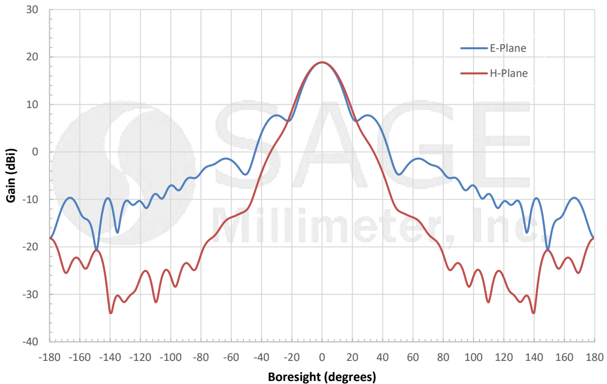
Simulated Antenna Patterns @ 40 GHz
