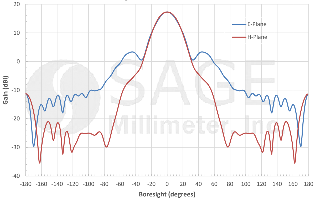
Simulated Antenna Patterns @ 60 GHz
