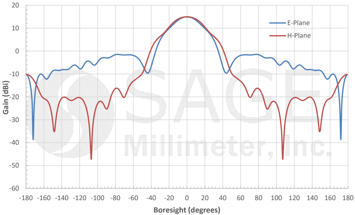
Simulated Antenna Patterns @ 40 GHz
