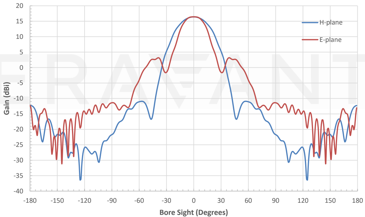
Simulated Antenna Pattern at 90 GHz
