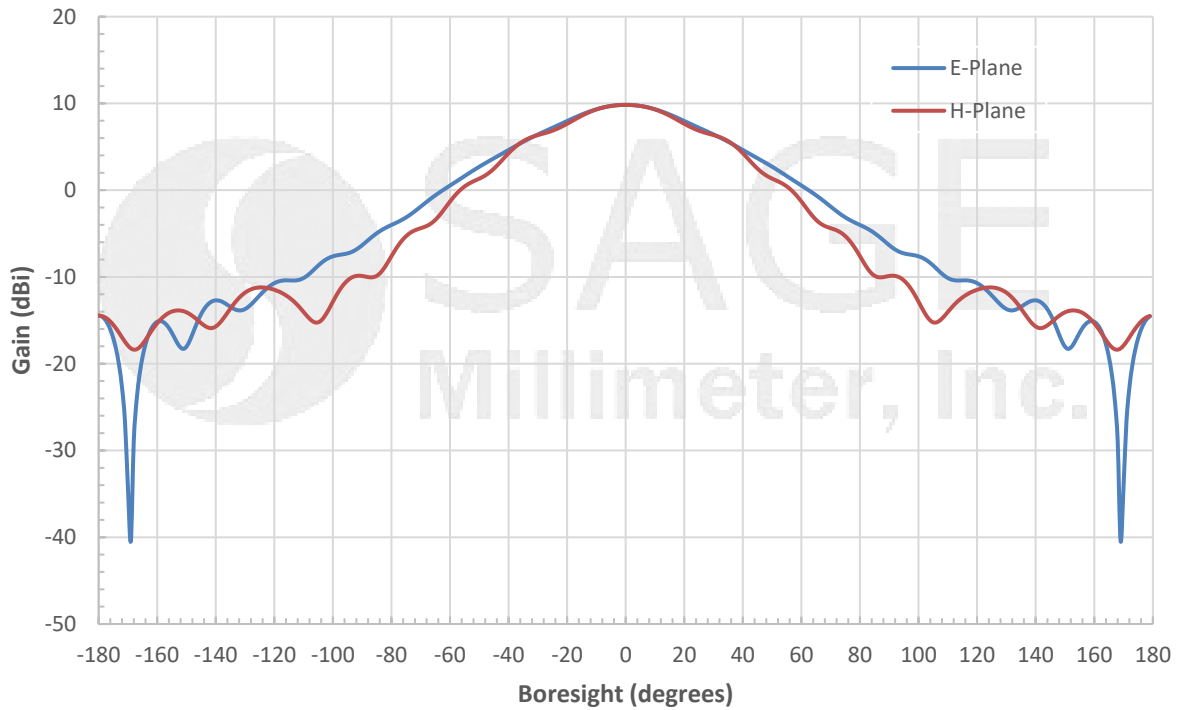
Simulated Antenna Patterns @ 50 GHz
