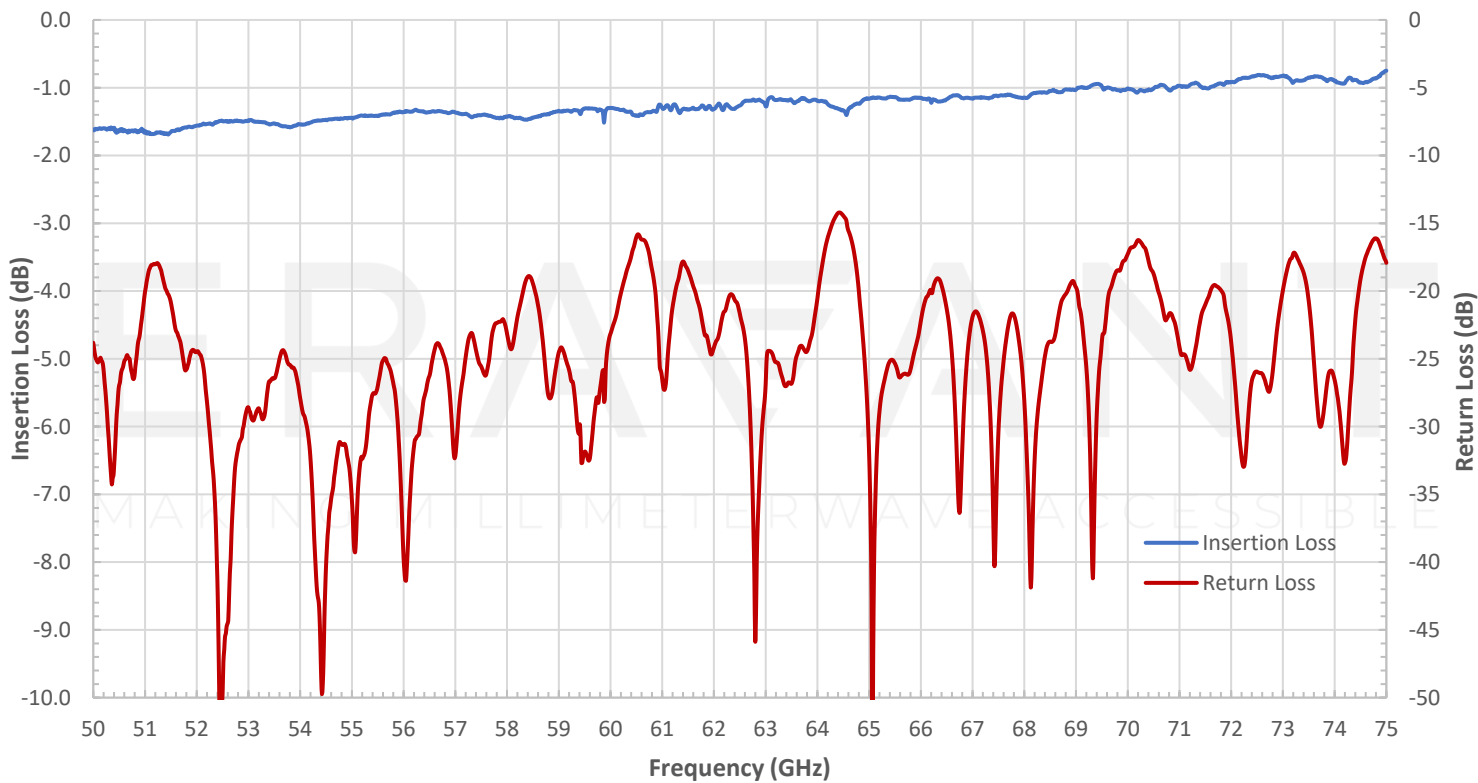
Typical Measured Insertion Loss and Return Loss vs. Frequency
