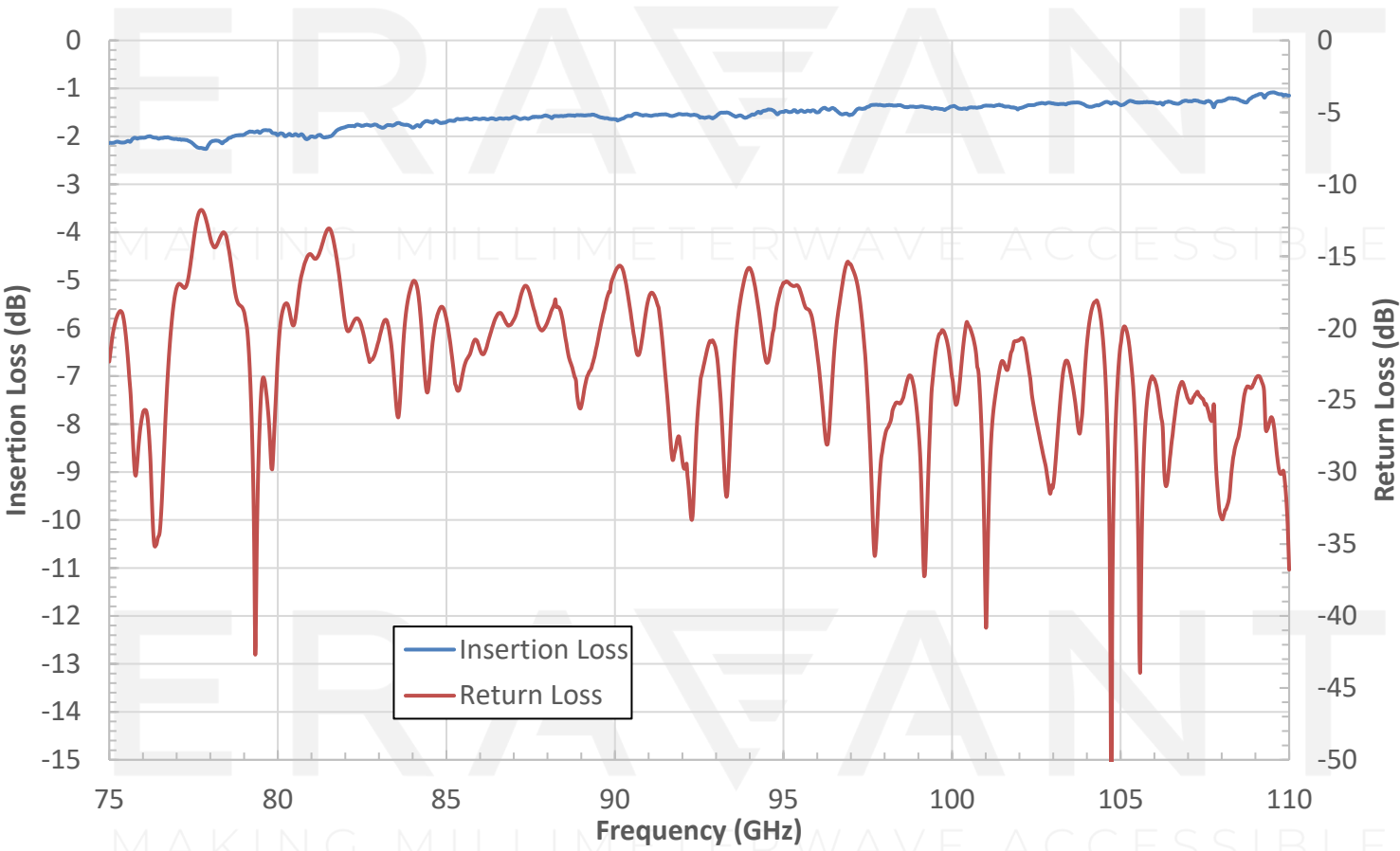
Typical Measured Insertion Loss and Return Loss vs. Frequency
