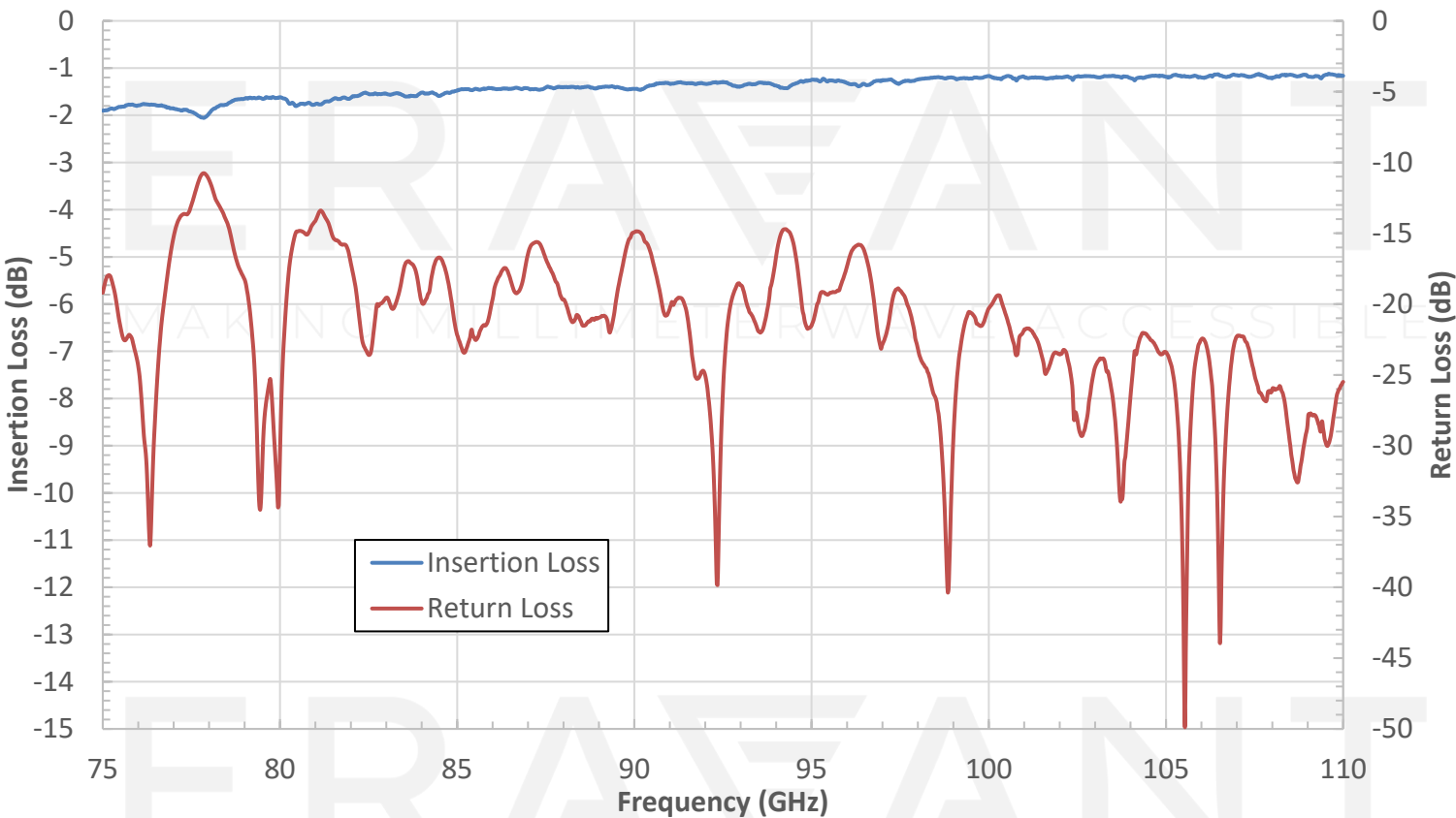
Typical Measured Insertion Loss and Return Loss vs. Frequency
