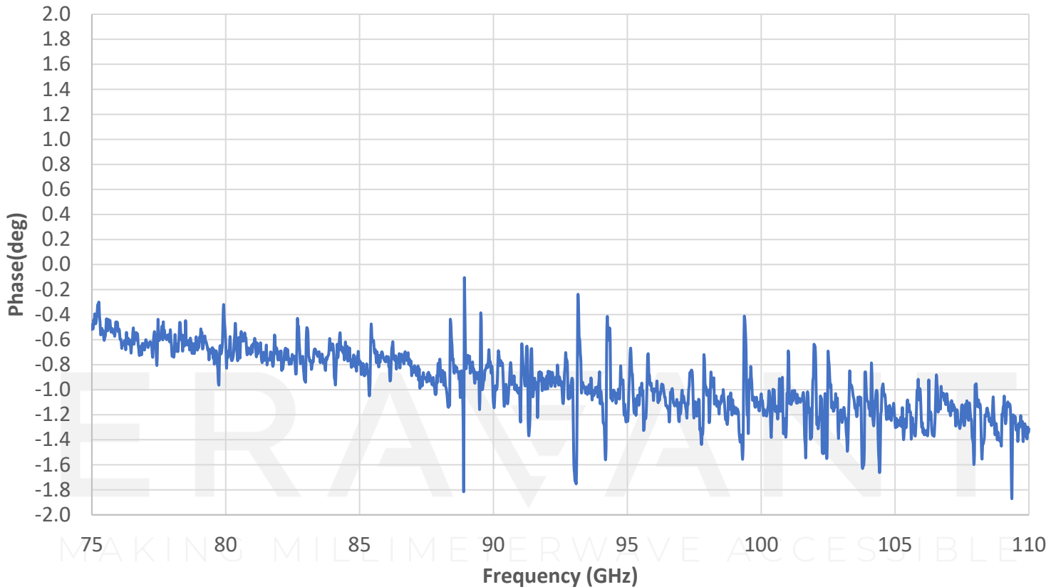
Typical Measured Phase Variance vs. Frequency
