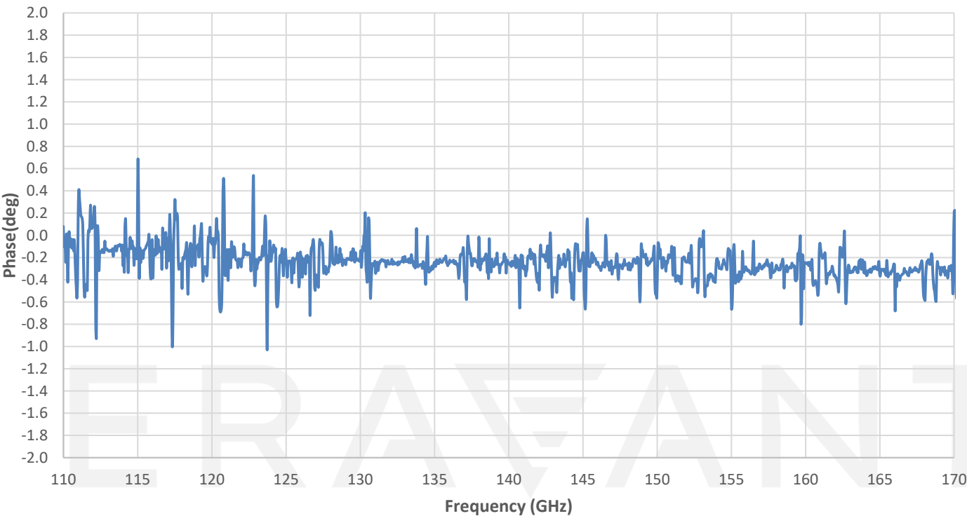
Typical Measured Phase Variance vs. Frequency
