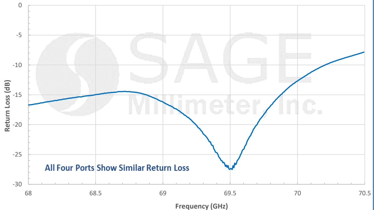
Measured Individual Patch Return Loss vs. Frequency
