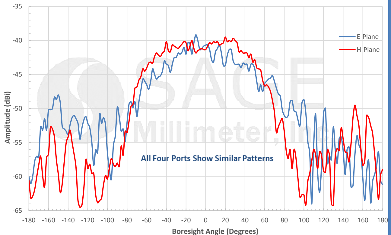
Measured Individual Patch Pattern @ 69.17 GHz
