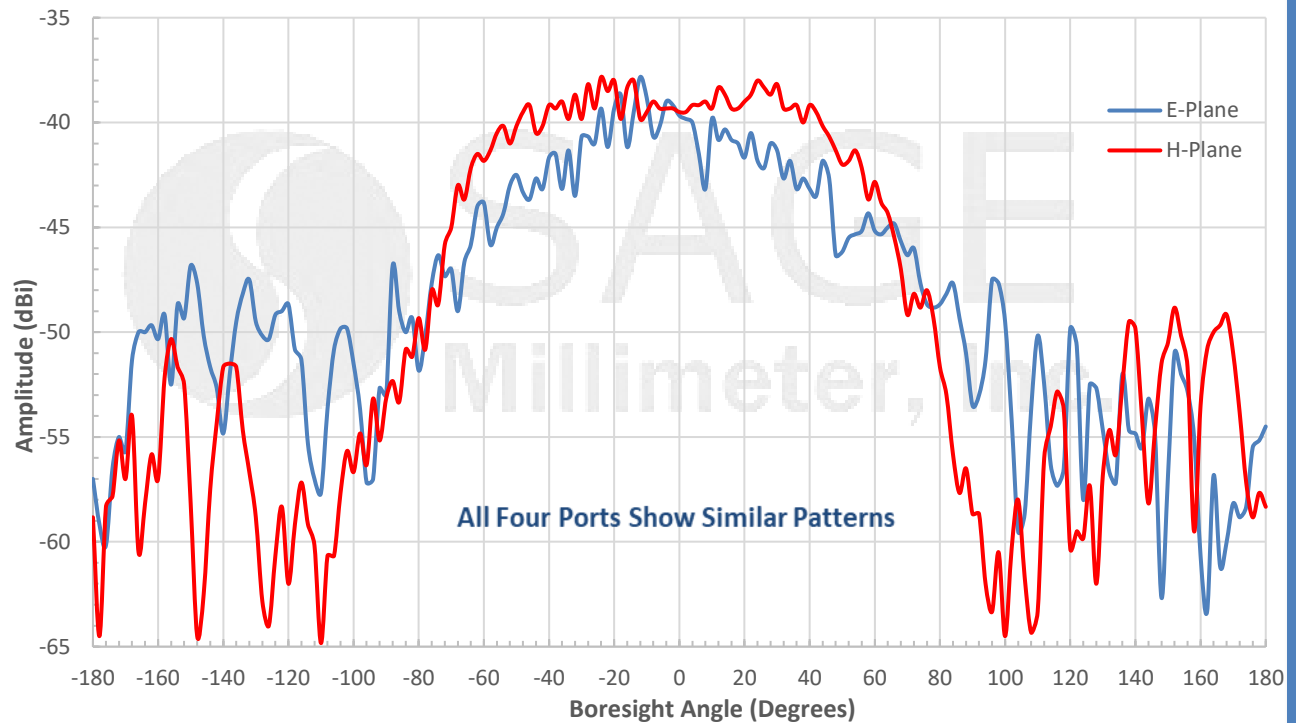
Measured Individual Patch Pattern @ 69.17 GHz
