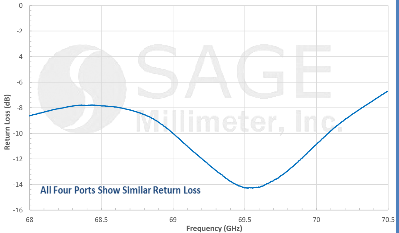
Measured Individual Patch Return Loss vs. Frequency
