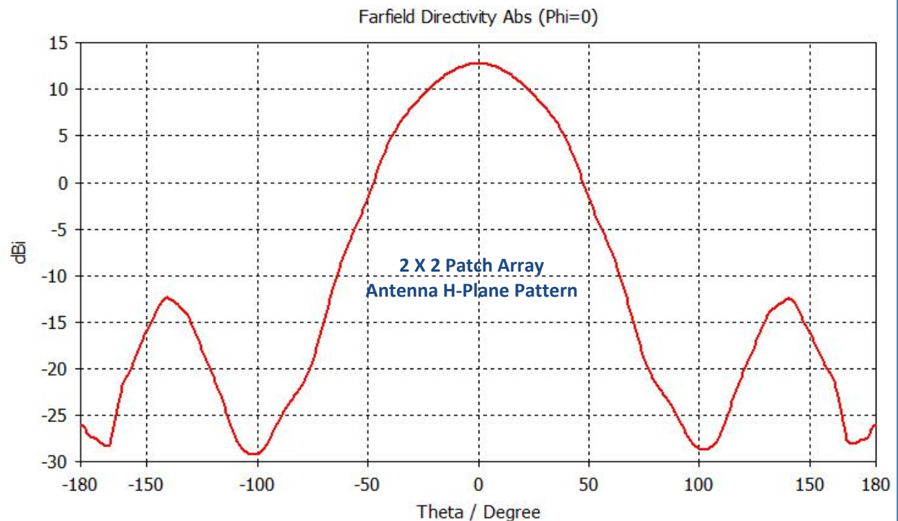
In-Phase Fed Simulated H-Plane Patch Array Antenna Pattern @ 67 GHz
