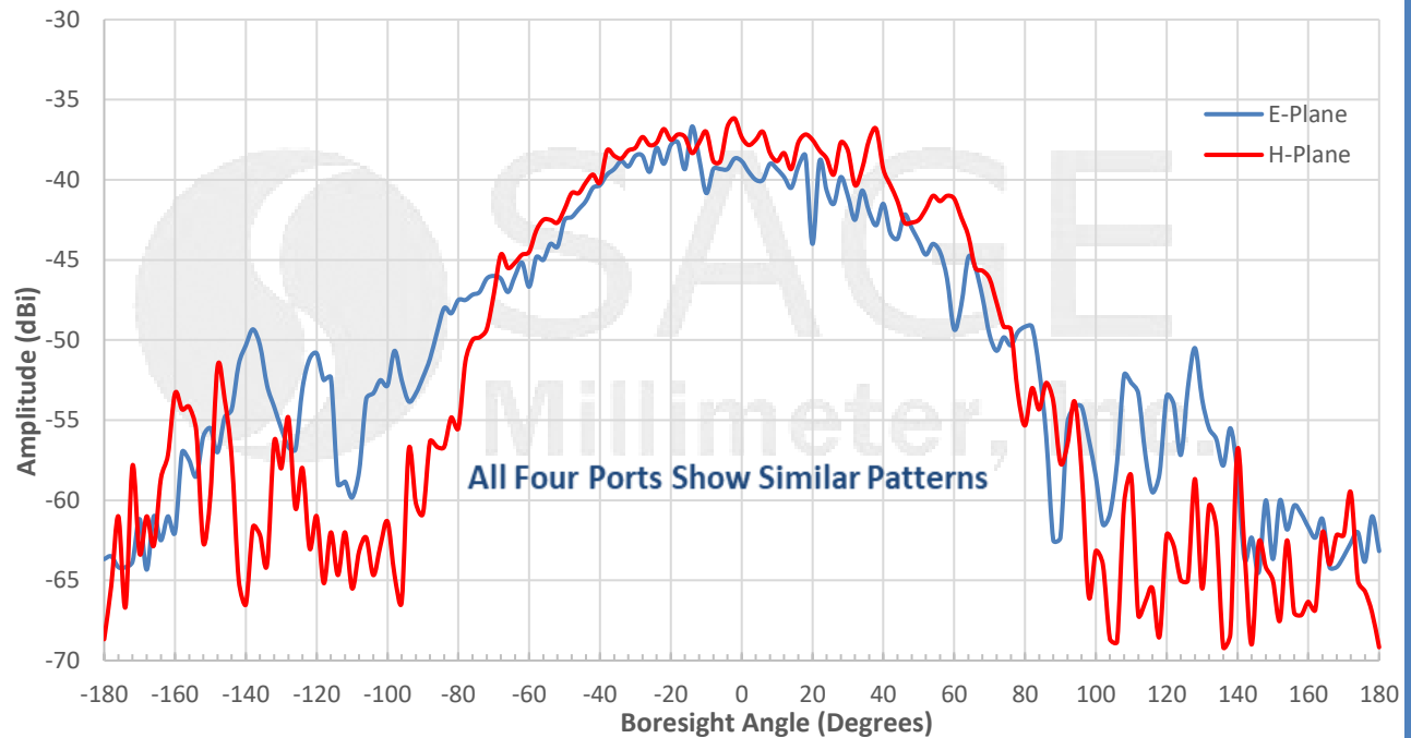
Measured Individual Patch Pattern @ 66.96 GHz
