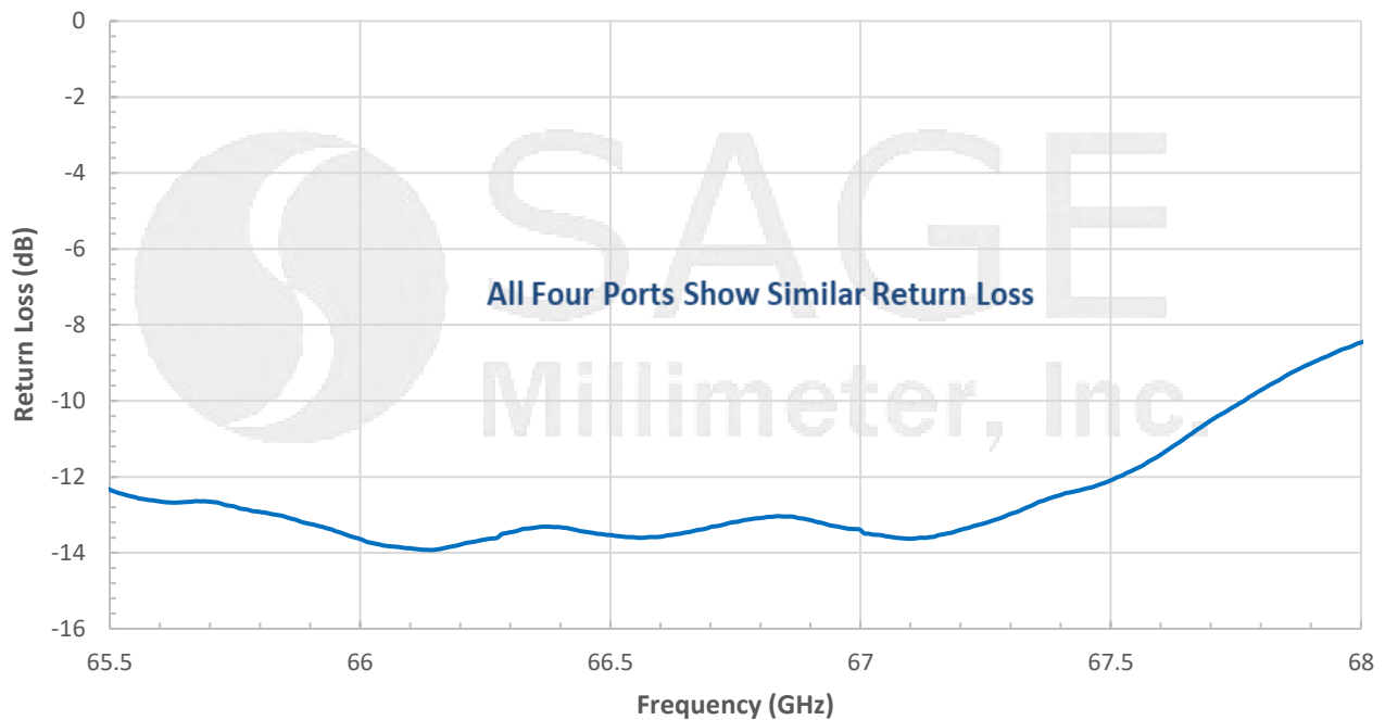
Measured Individual Patch Return Loss vs. Frequency
