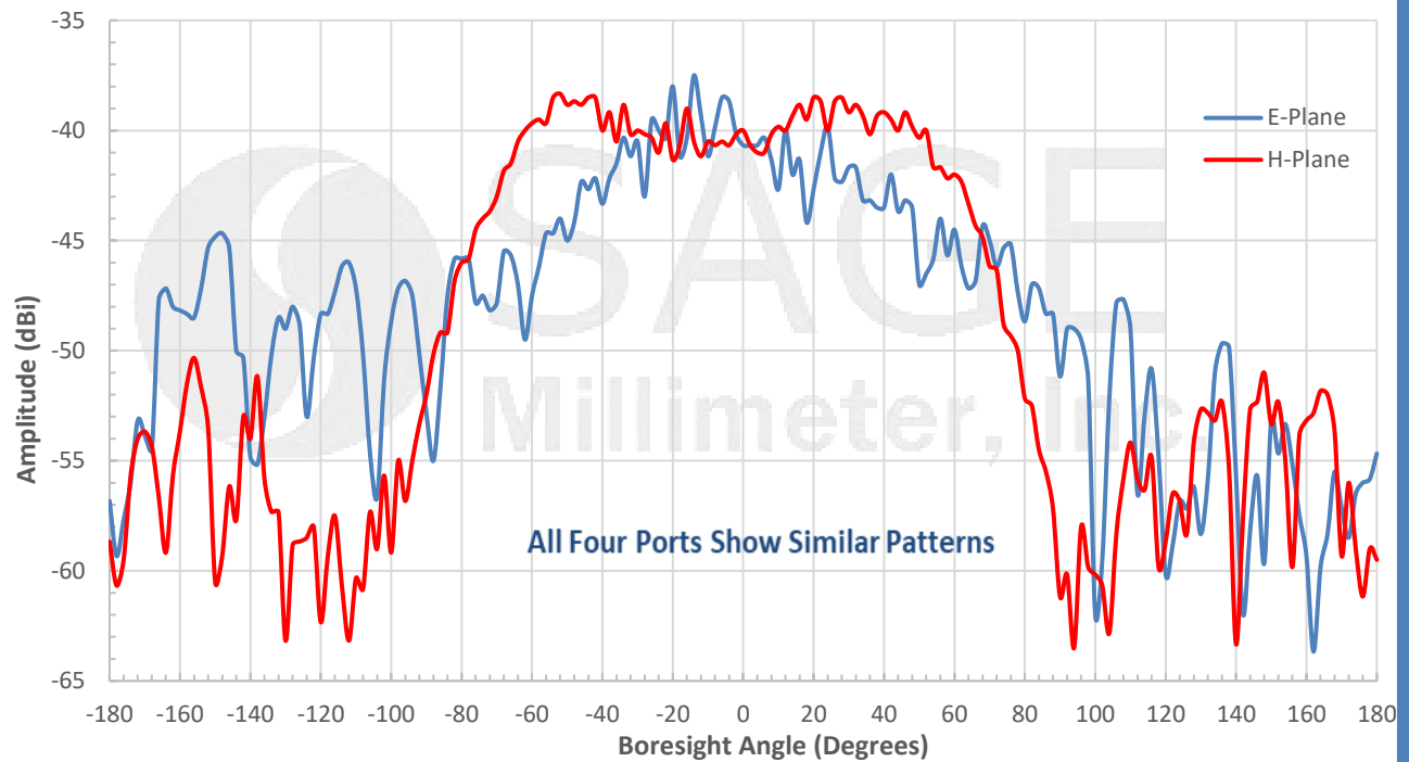
Measured Individual Patch Pattern @ 66.96 GHz
