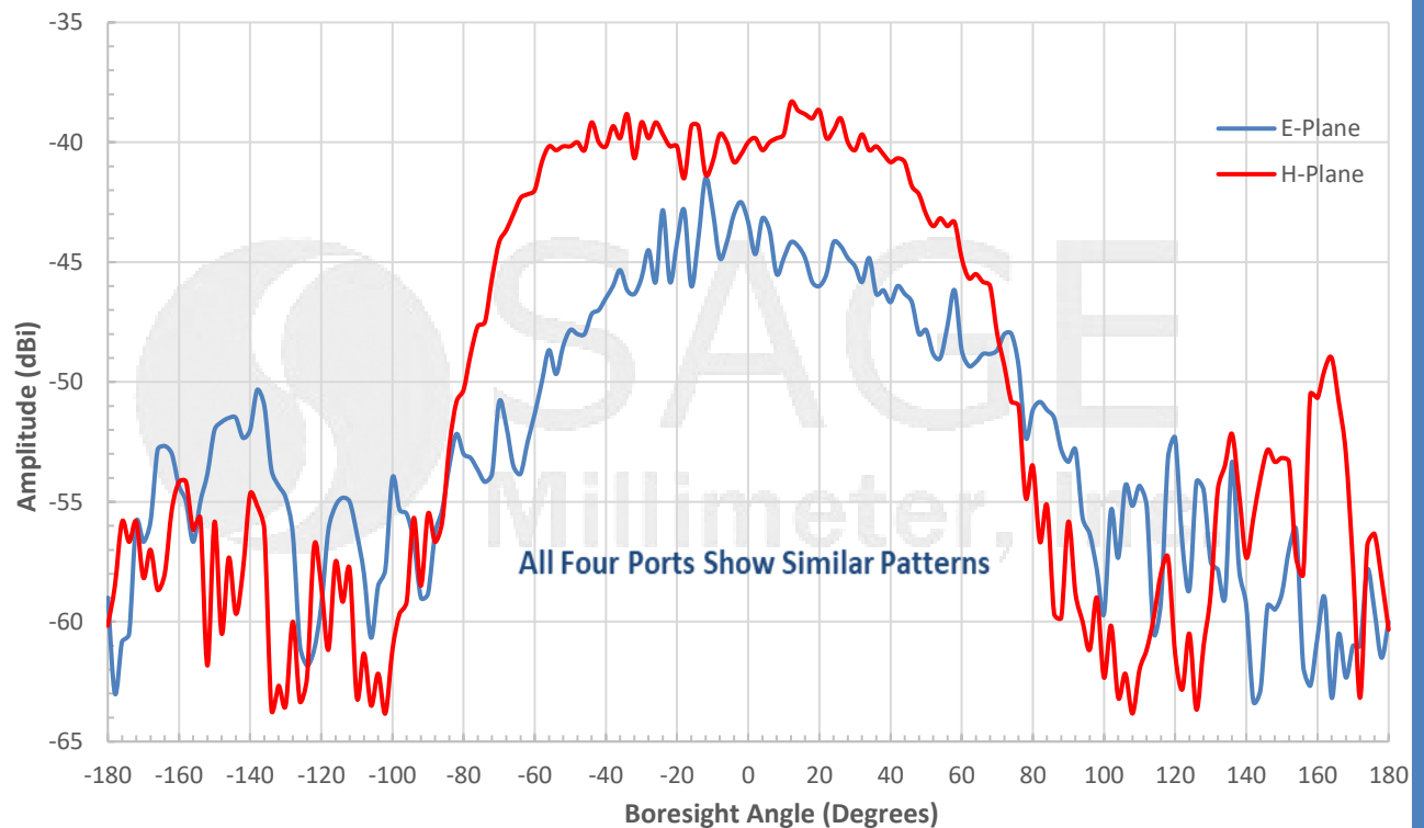
Measured Individual Patch Pattern @ 66.96 GHz
