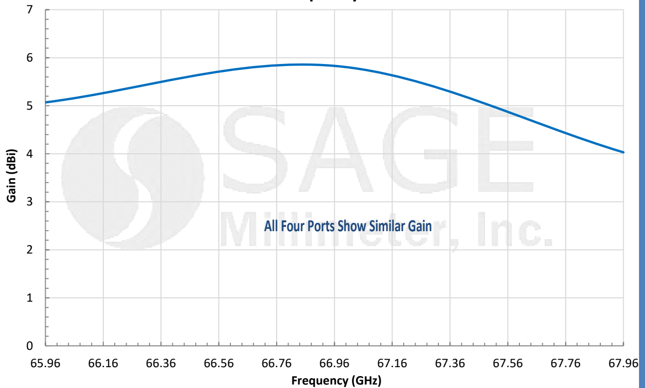
Measured Individual Patch Gain vs. Frequency
